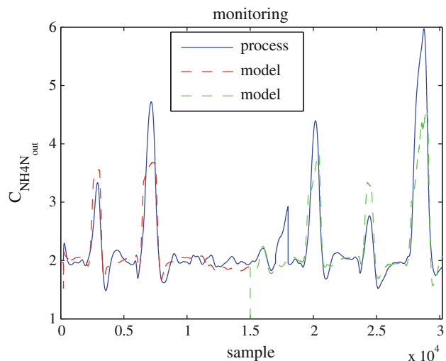
Fig. 5 The monitoring. The model output and the process output for the whole measurement set
