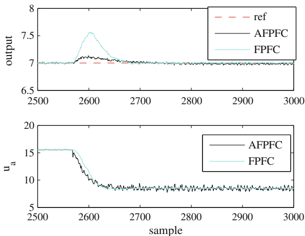
Fig. 11 Disturbance rejection
